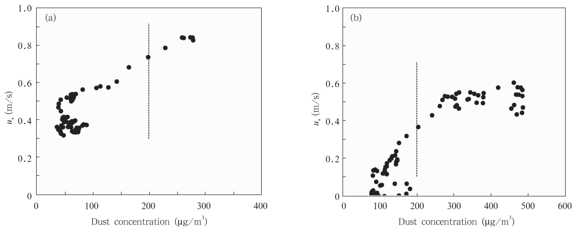
图 5 2006 年 4 月 10 日(a)和 14 日(b)黄土高原两次沙尘天气过程中沙尘浓度与摩擦速度的变化 Fig. 5 Relationship between the dust concentration and the friction velocity during the dust events on (a) 10 and (b) 14 April 2006 over the Loess Plateau
