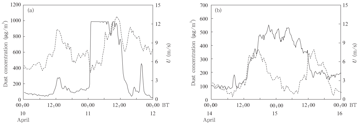
图 4 2006年4月10—11日(a)和14—15日(b)黄土高原沙尘浓度(实线)与风速(虚线)的时间变化 Fig. 4 Time series of the dust concentration (solid line) and the wind speed (dashed line) during (a) 10—11 and (b) 14—15 April 2006 over the Loess Plateau
