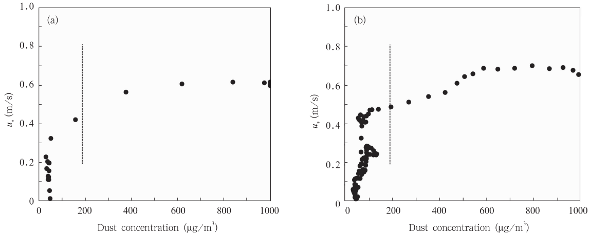
图 7 2006 年 4 月 10 日(a)和 28 日(b)戈壁地区两次沙尘天气过程中沙尘浓度与摩擦速度的变化 Fig. 7 Relationship between the dust concentration and the friction velocity during the dust events on (a) 10 and (b) 28 April 2006 over the Gobi area
