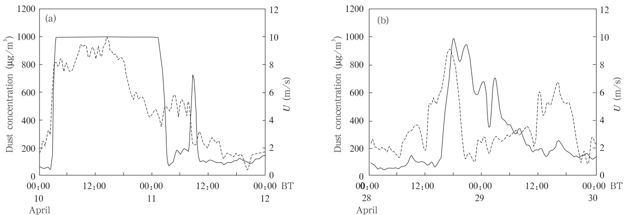
图 6 2006 年 4 月 10—11 日(a)和 28—29 日(b)戈壁地区沙尘浓度(实线)与风速(虚线)的时间变化 Fig. 6 Time series of the dust concentration (solid line) and the wind speed (dashed line) during (a) 10-11 and (b) 28-29 April 2006 over the Gobi area
