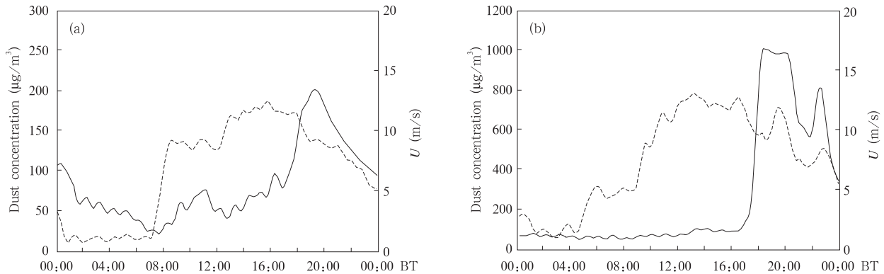
图2 2004年3月16日(a)和27日(b)浑善达克沙地沙尘浓度(实线)和风速(虚线)的日变化 Fig.2 Diurnal variation of the dust concentration (solid line) and the wind speed (dashed line) on (a) 16 and (b) 27 March 2004 over the Hunshandake desert area
